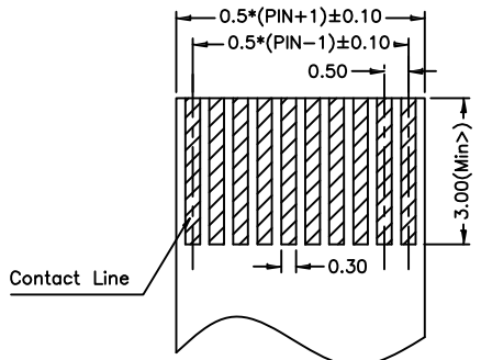
Thickness: 0.30±0.03 FPC Dimension Reference
