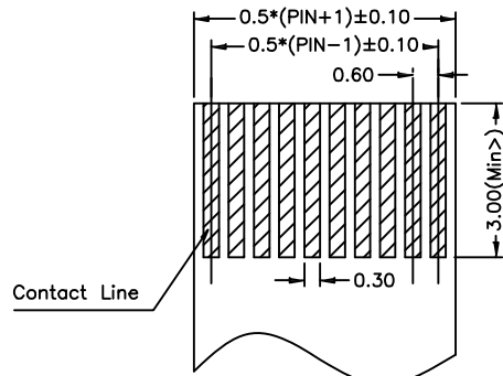
Thickness: 0.30±0.03 FPC Dimension Reference
